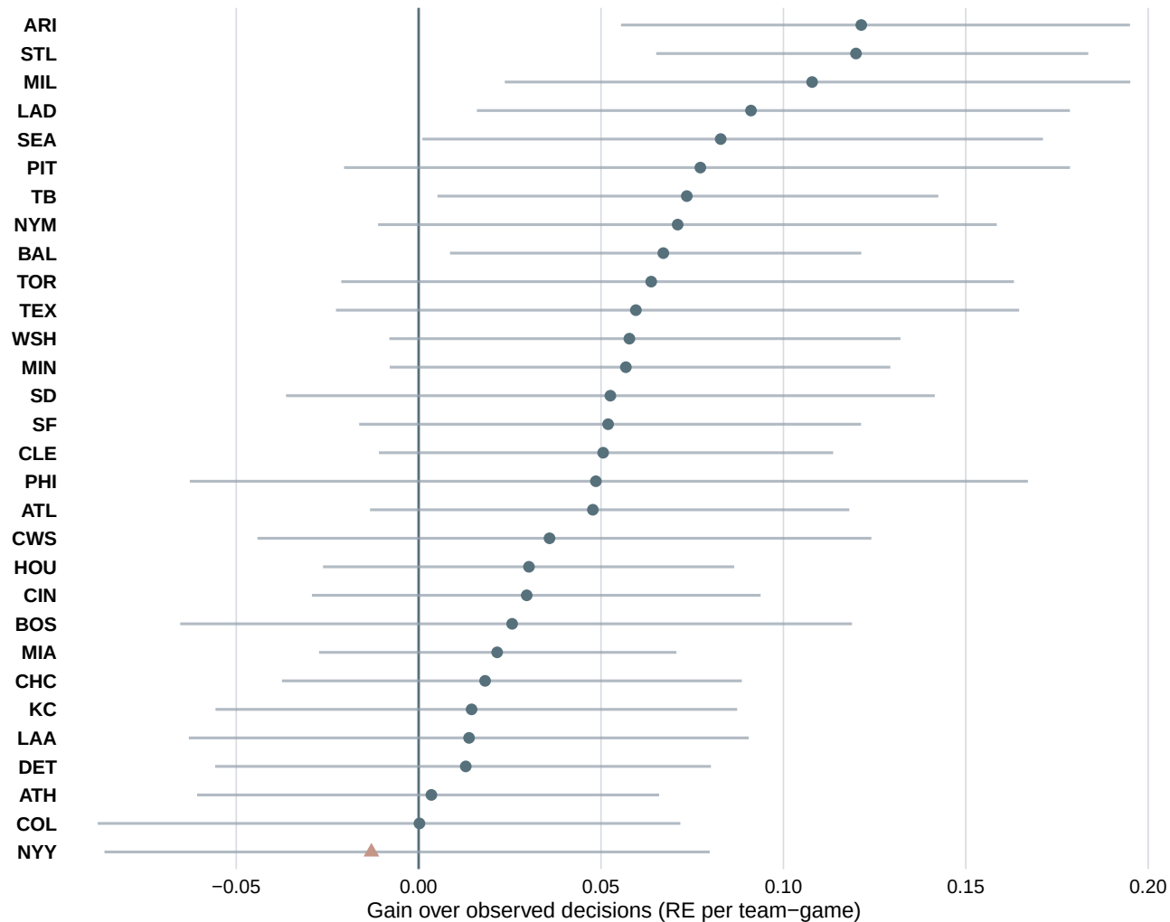
Estimated policy gains vary across teams
