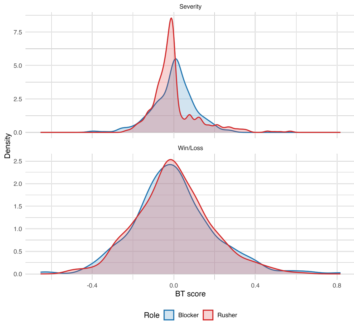
Figure 1: Distribution of raw BT scores by model and role. Higher scores indicate stronger performance within role.
