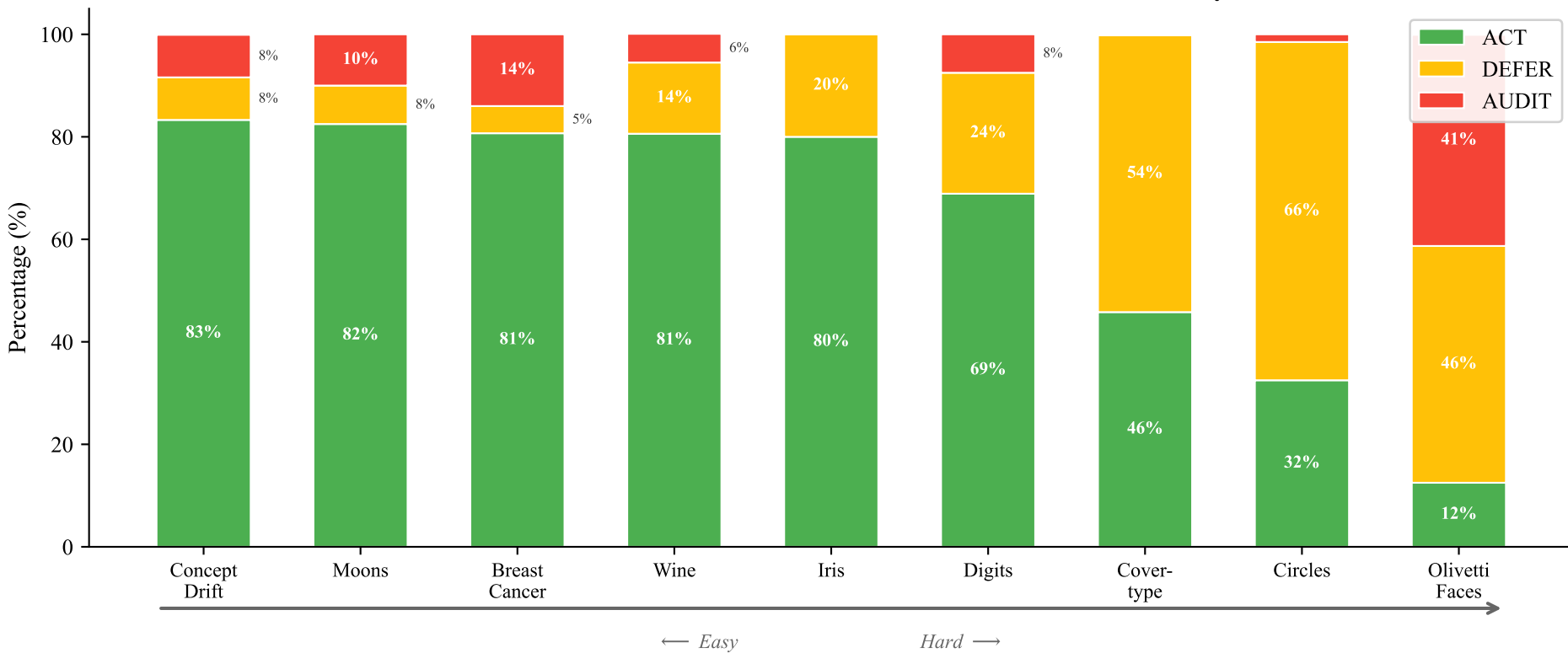
CRC Decision Gate Breakdown: ICM Scales with Problem Difficulty
