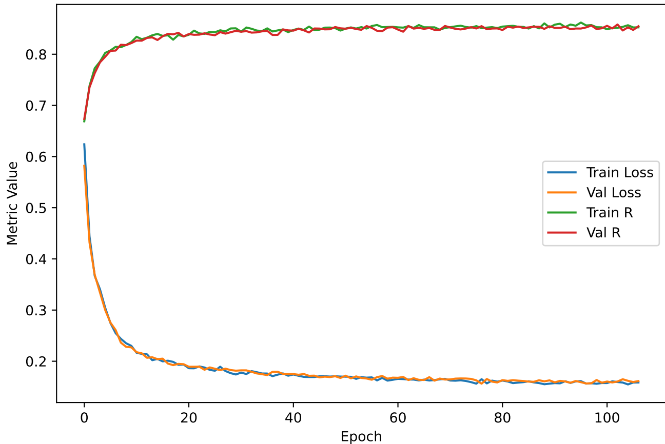
ATAC MAE (Masked MSE + PearsonR)
