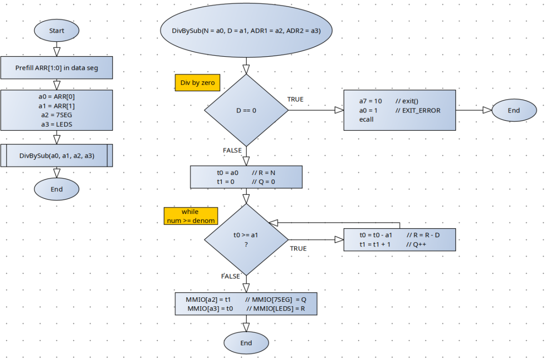
Figure 59: Flow chart for part 1
