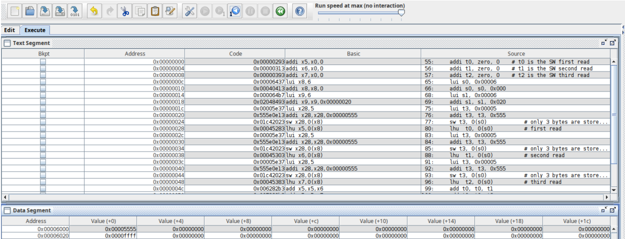
Figure 27: Data segment after executing instructions
