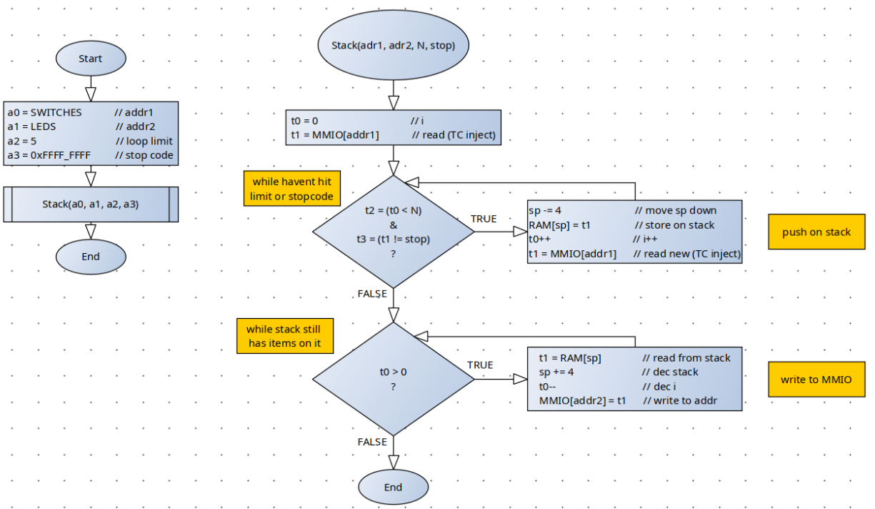
Figure 60: Flow chart for part 2
