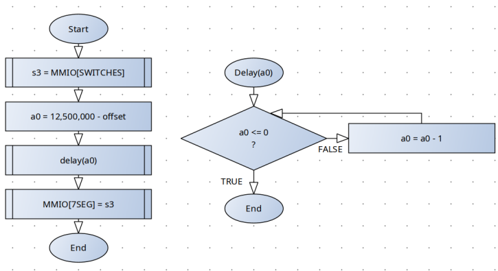
Figure 52: Flow chart for part 2
