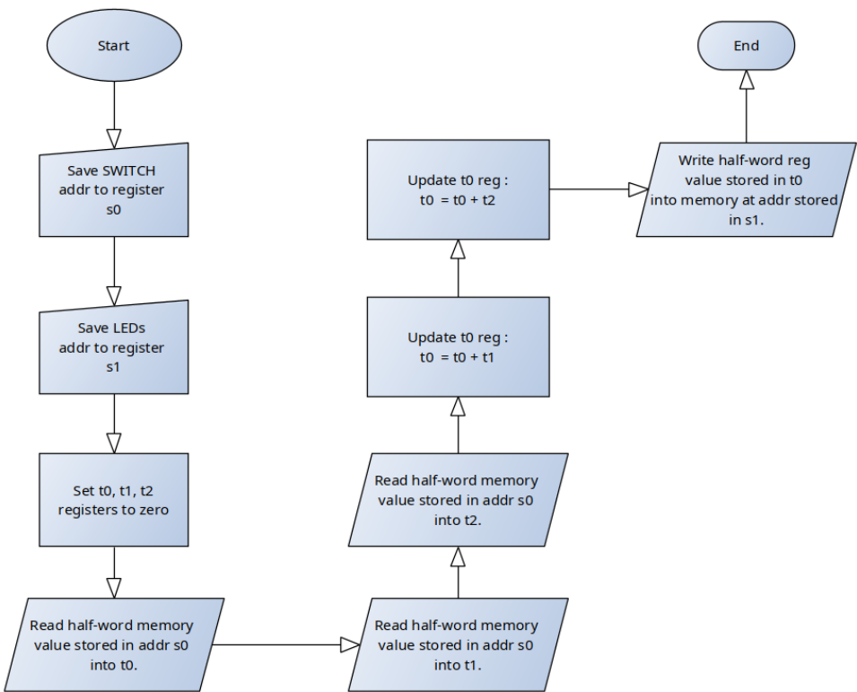
Figure 20: Flow Chart for Part 1
