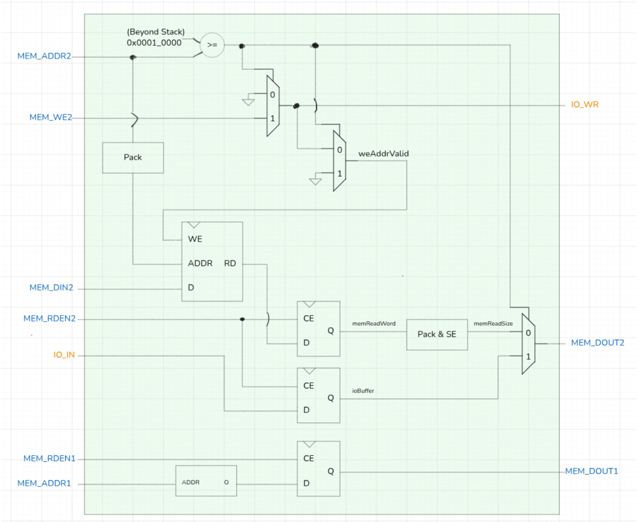
Figure 18: Flow Diagram for Memory
