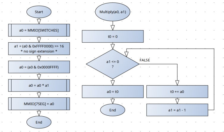
Figure 51: Flow chart for part 1
