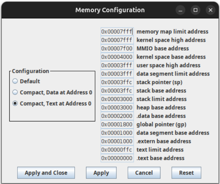
Figure 54: Memory Map for this Assignment
