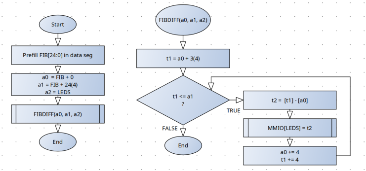
Figure 55: Flow chart for part 1
