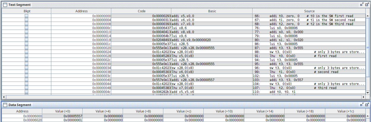
Figure 21: Data segment after executing instructions
