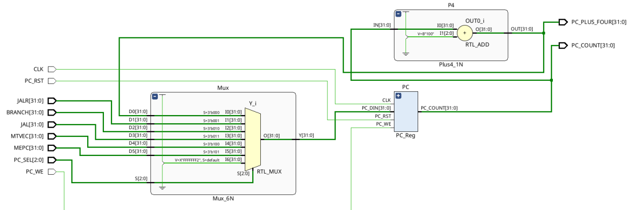
Figure 7: RTL Design of PC_TestBlock.sv
