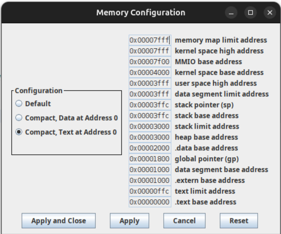
Figure 1: RARS Memory Config Settings
