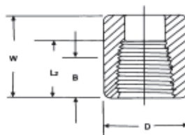
Half-Coupling
