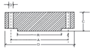
BLIND FLANGE
