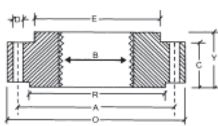
THREADED FLANGES
