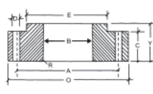
LAP JOINT FLANGES
