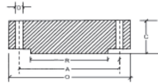
BLIND FLANGE
