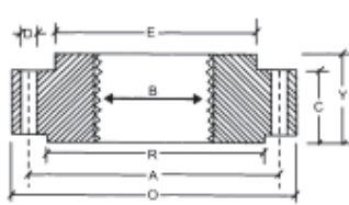
THREADED FLANGES
