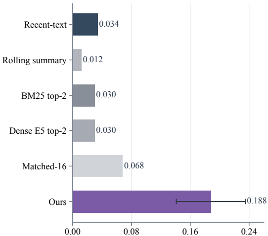
(a) Exact Match \uparrow
