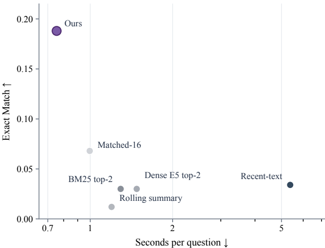
(a) Exact Match vs. Seconds per Question
