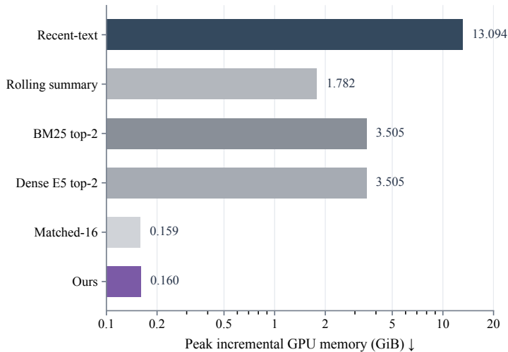
(b) Peak Incremental GPU Memory
