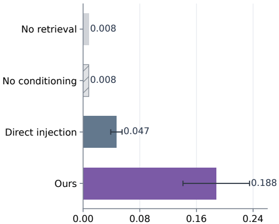
(a) Exact Match \uparrow
