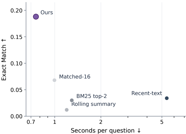
(a) Exact Match vs. Seconds per Question
