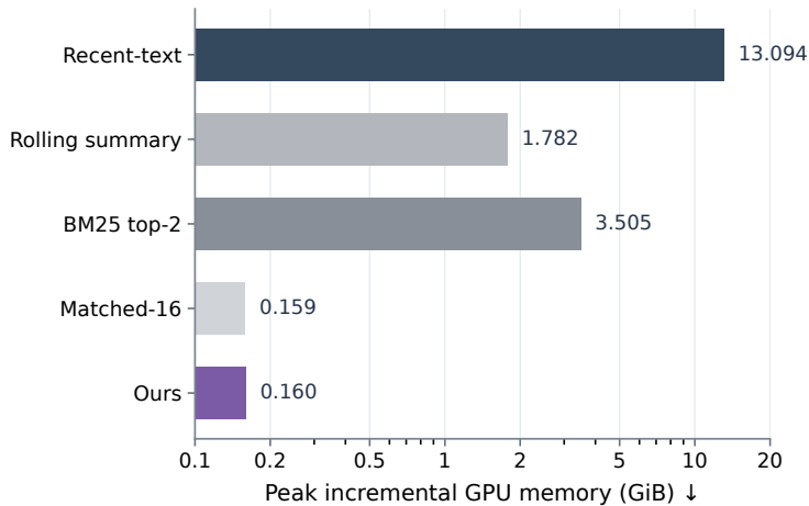
(b) Peak Incremental GPU Memory
