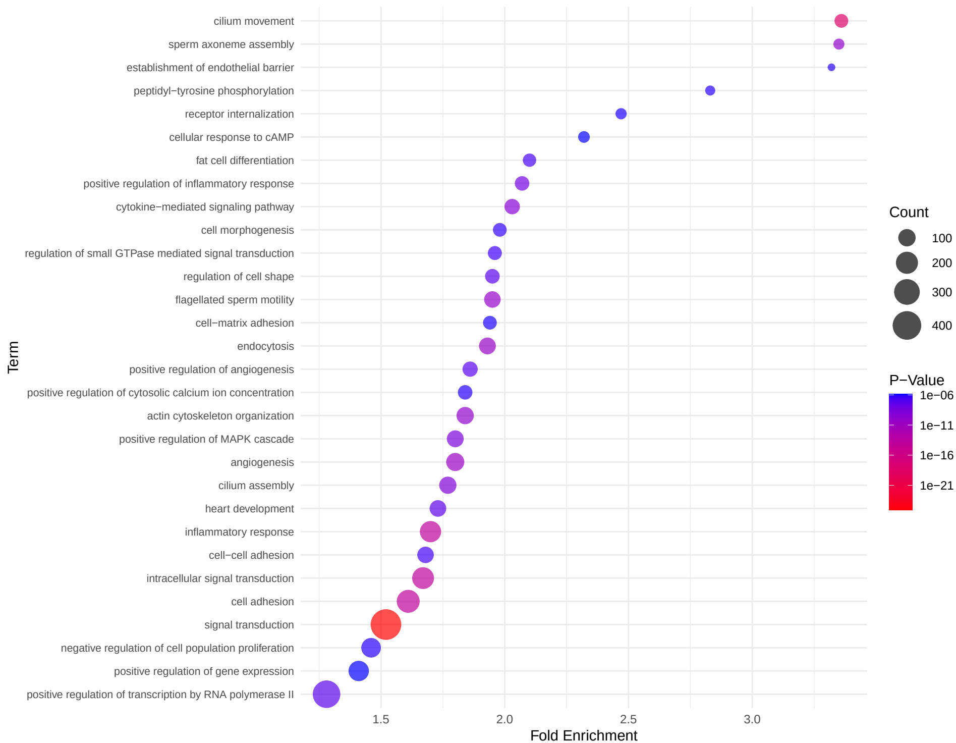
LUAD_AllRace_DownRegulated_BPDirect_Dotplot
