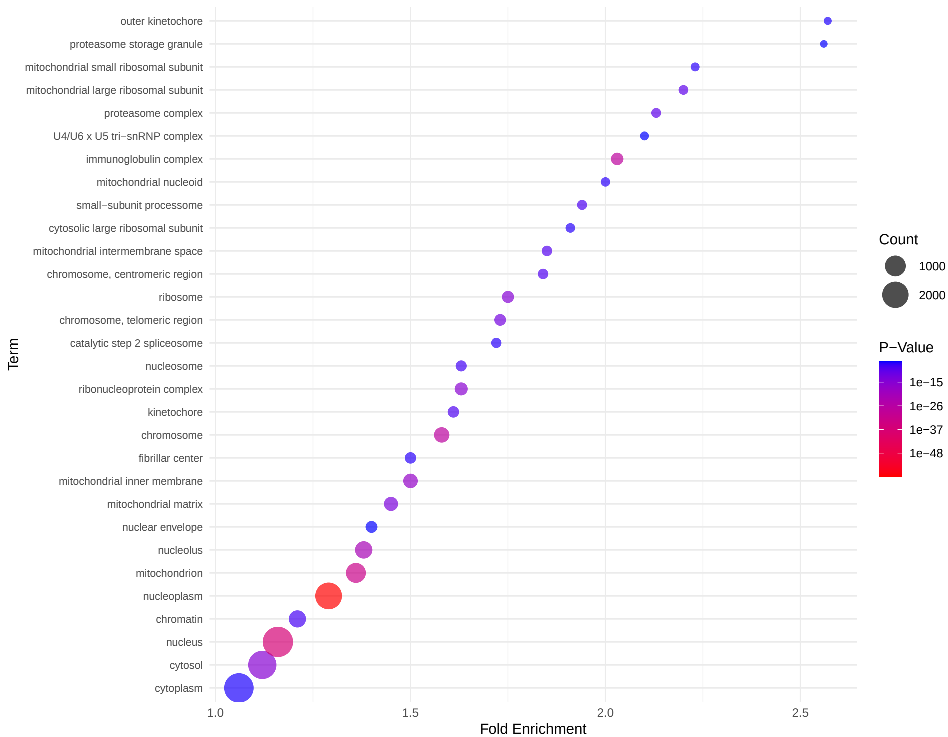
LUAD_AllRace_UpRegulated_CCDirect_Dotplot
