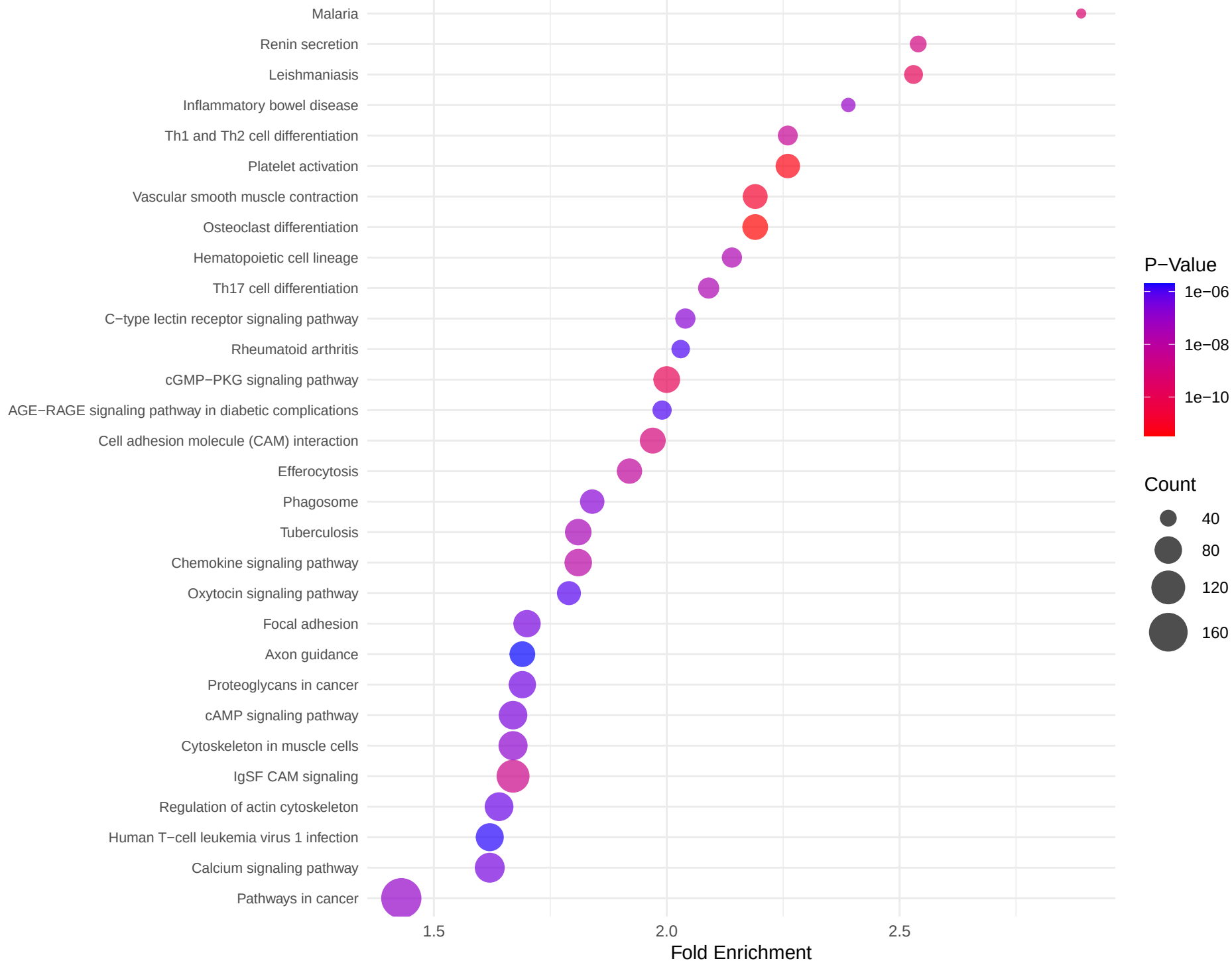
LUAD_AllRace_DownRegulated_KEGG_Dotplot
