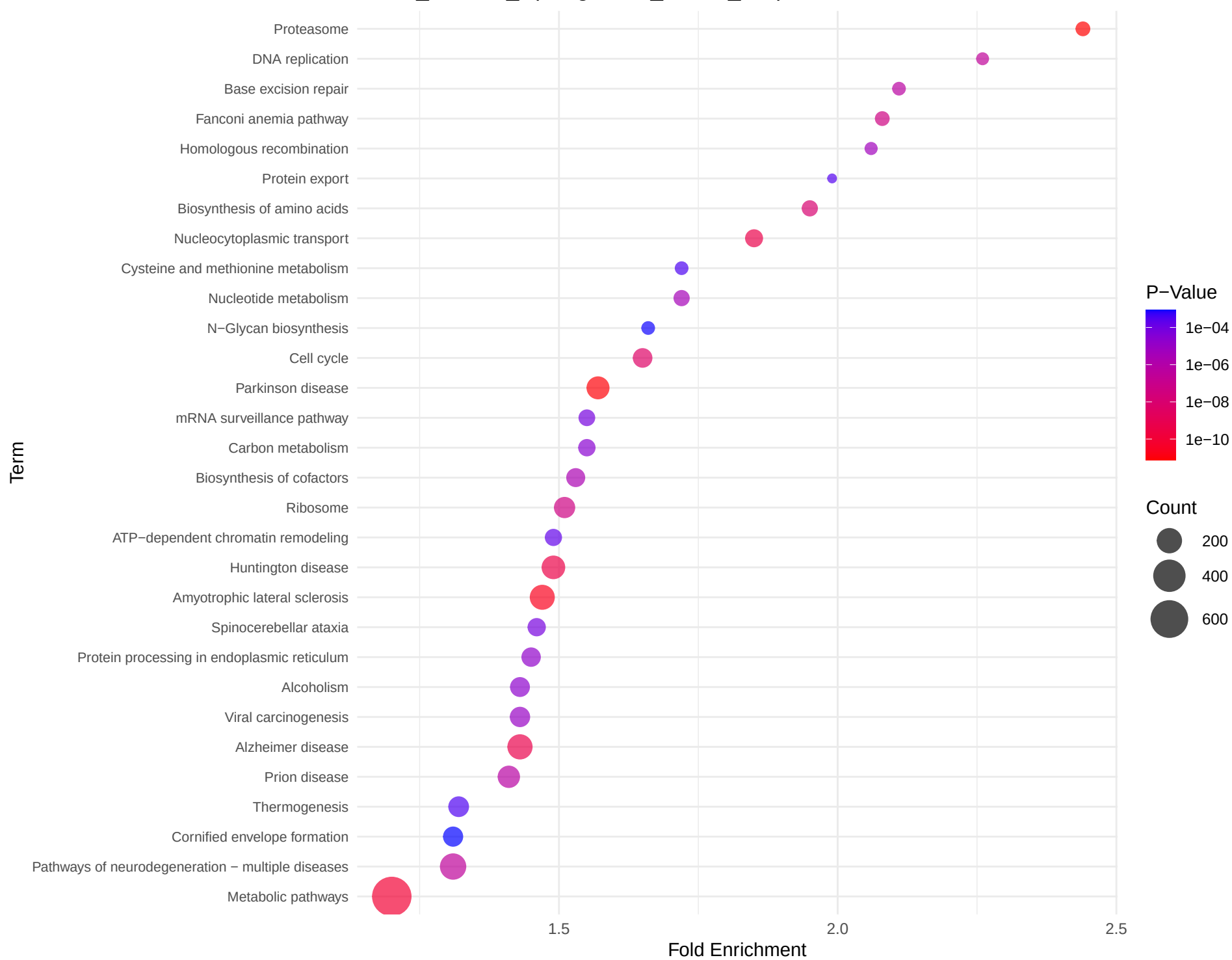
LUAD_AllRace_UpRegulated_KEGG_Dotplot
