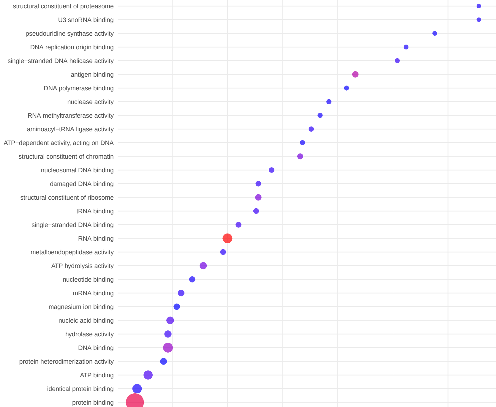
LUAD_AllRace_UpRegulated_MFDirect_Dotplot
