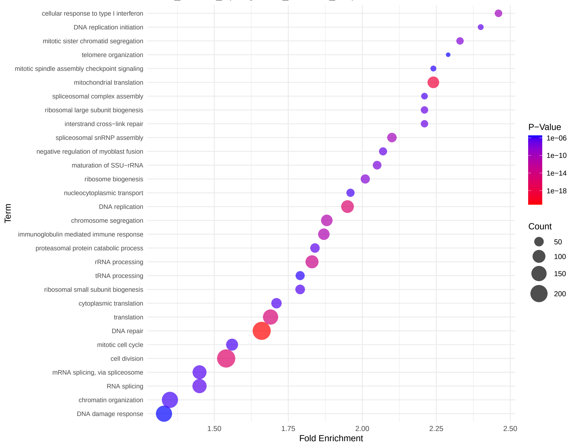
LUAD_AllRace_UpRegulated_BPDirect_Dotplot
