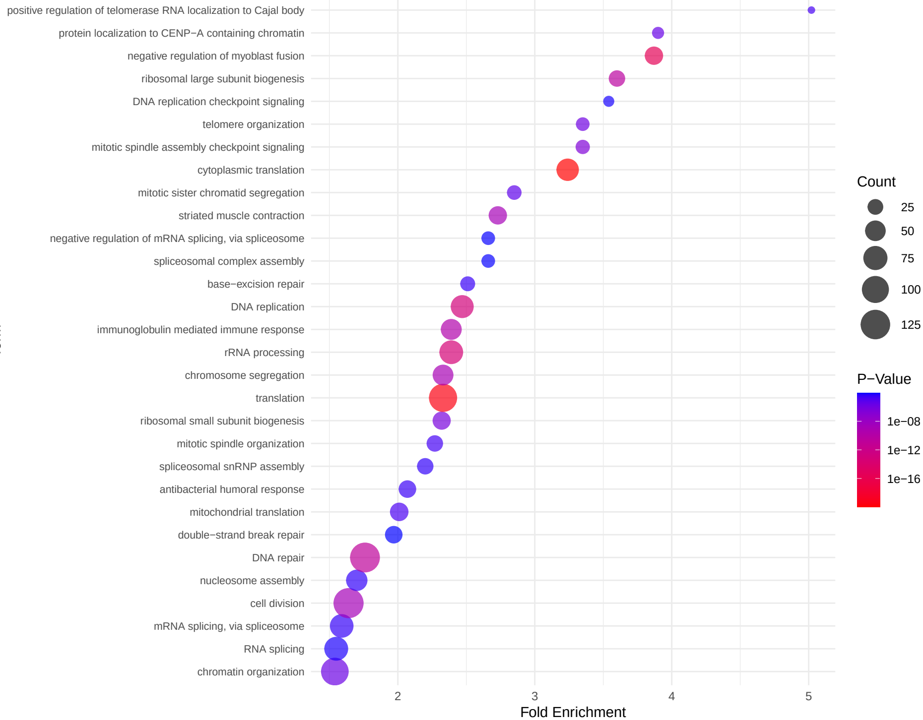
PRAD_WhiteRace_UpRegulated_BPDirect_Dotplot
