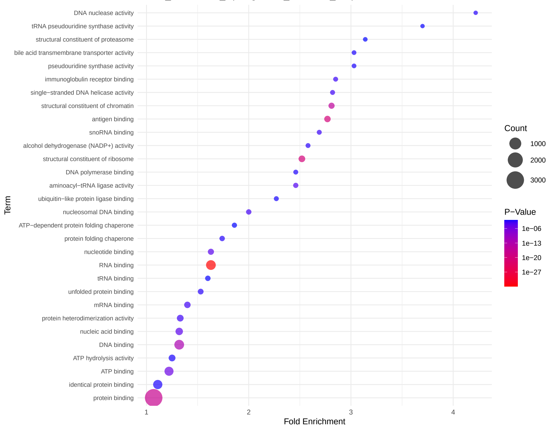
PRAD_WhiteRace_UpRegulated_MFDirect_Dotplot
