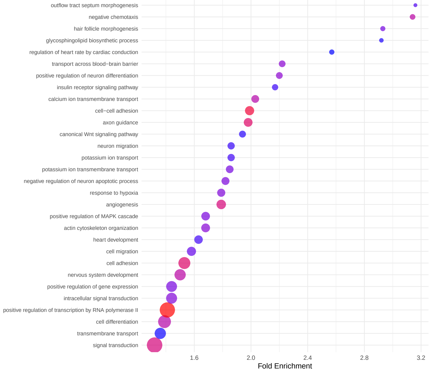
PRAD_WhiteRace_DownRegulated_BPDirect_Dotplot
