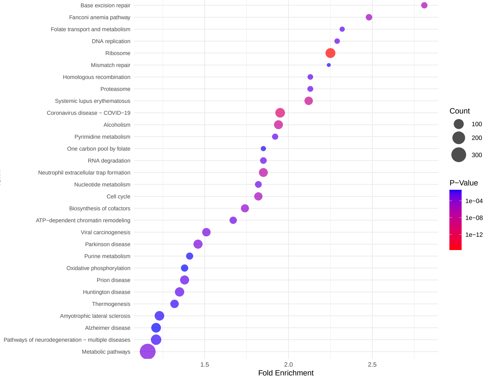
PRAD_WhiteRace_UpRegulated_KEGG_Dotplot
