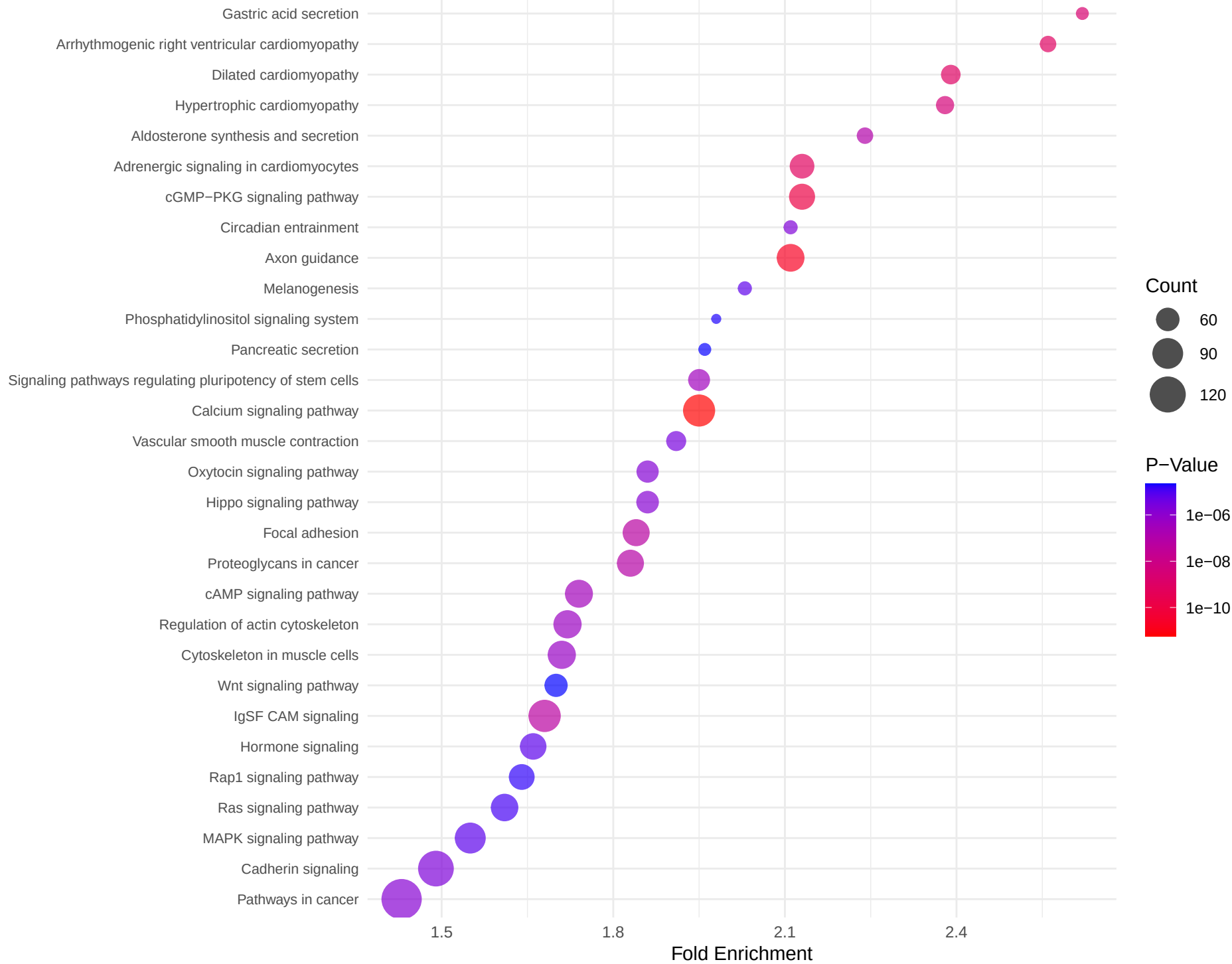
PRAD_WhiteRace_DownRegulated_KEGG_Dotplot
