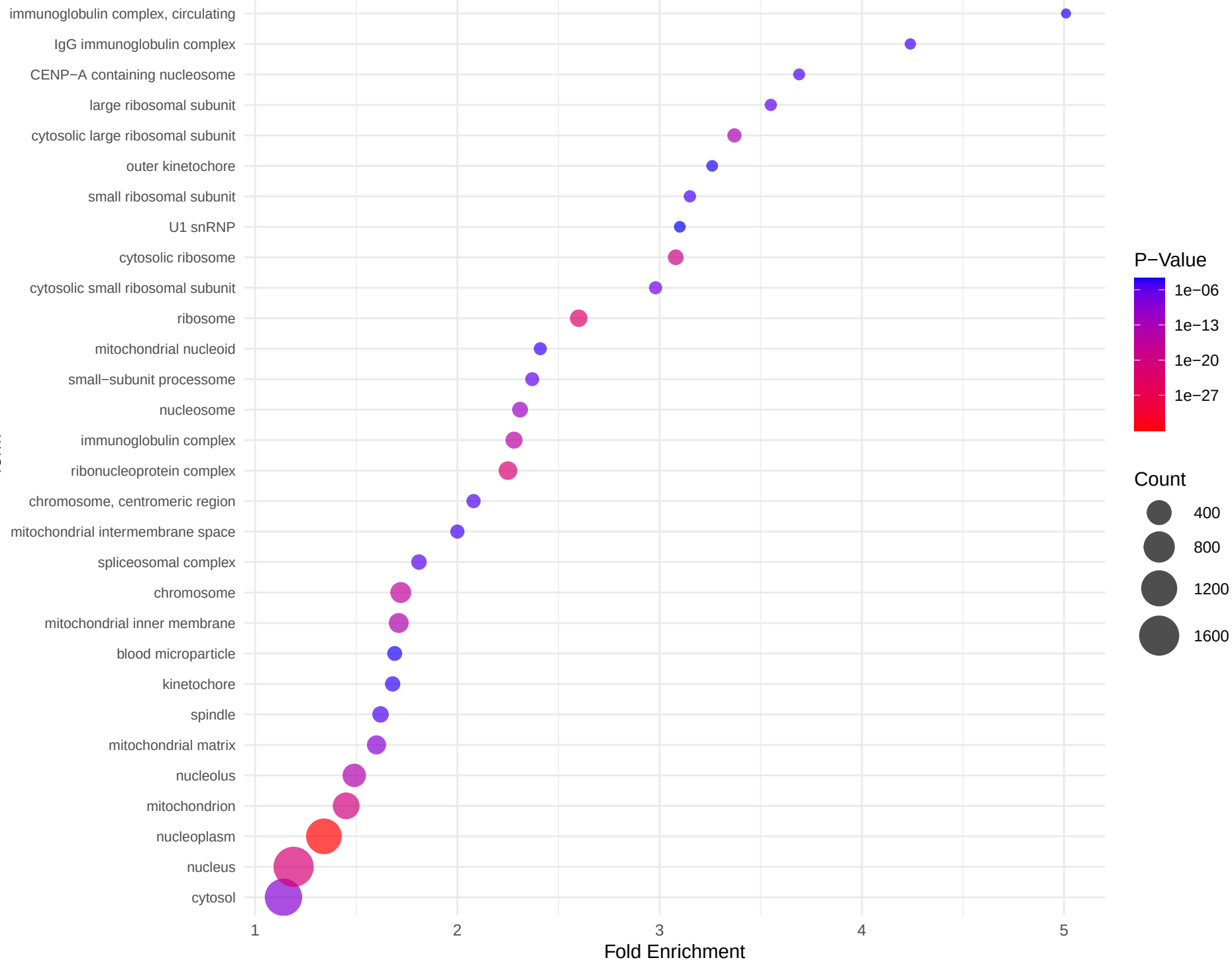
PRAD_WhiteRace_UpRegulated_CCDirect_Dotplot
