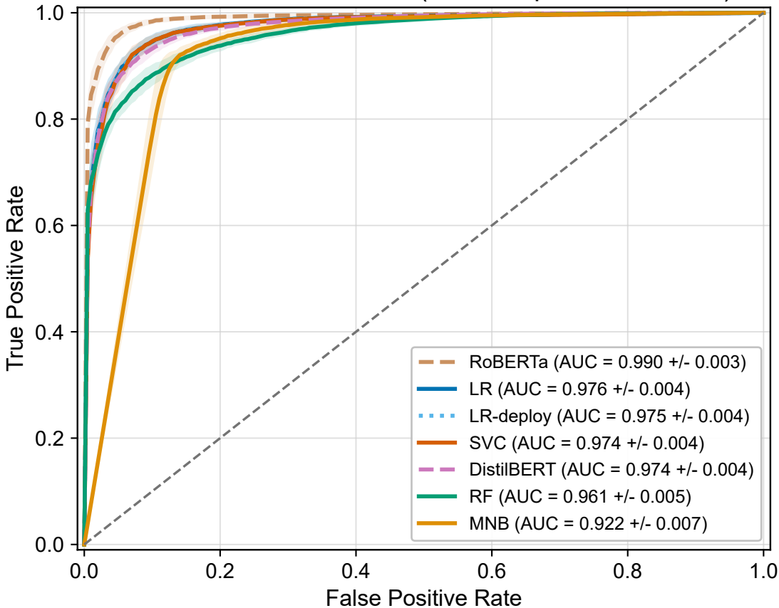
ROC Curves - All Models (Joint Corpus, 30-Run CV)
