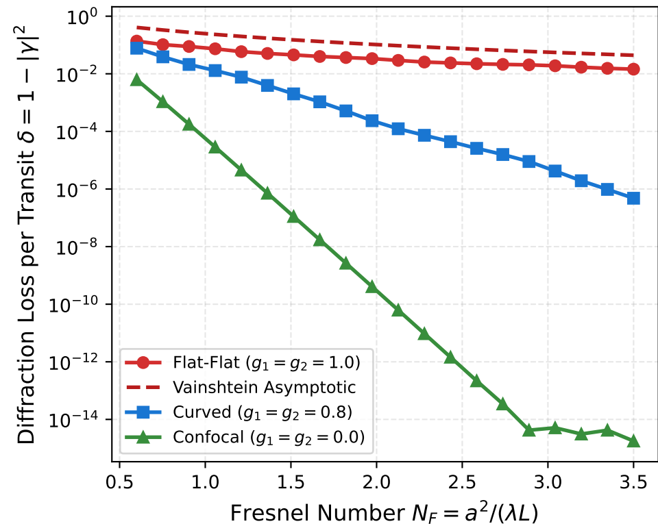
(a) Diffraction Loss vs N_F
