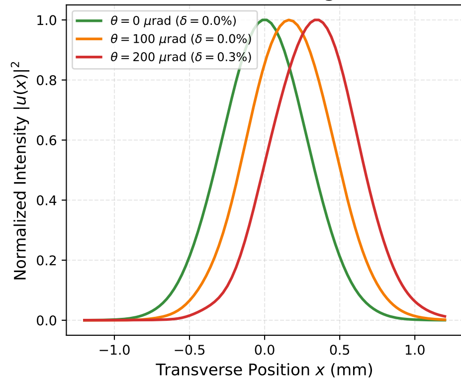
(c) Mirror Tilt Misalignment
