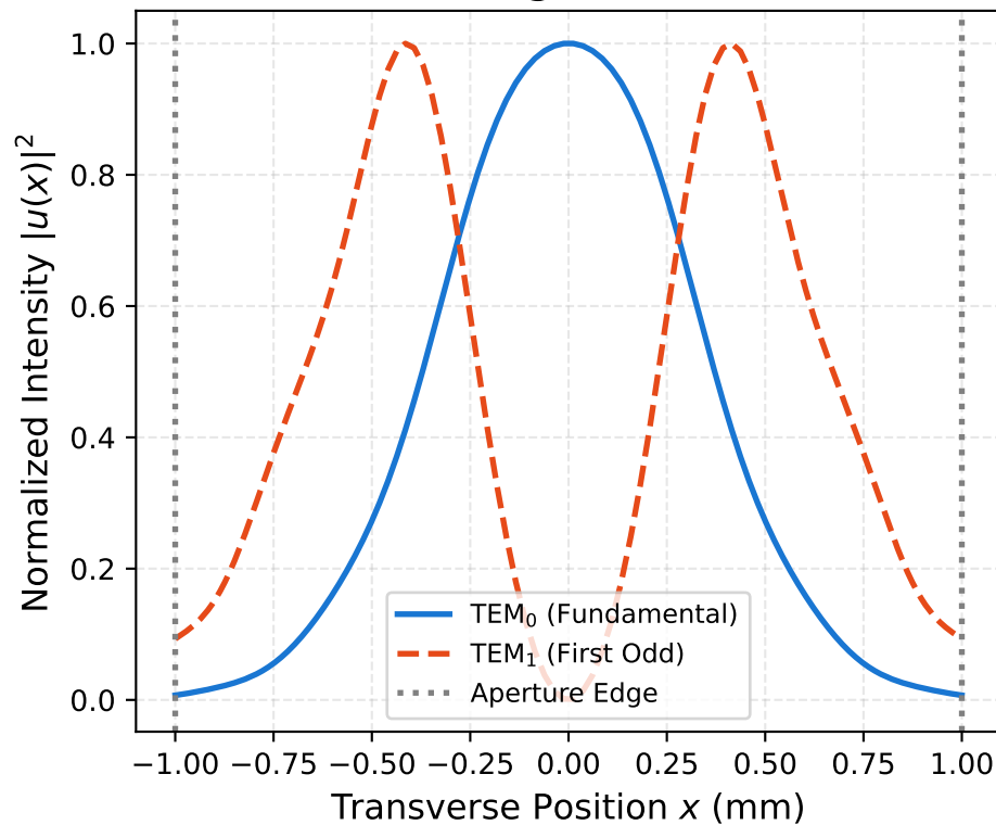
(b) Transverse Eigenmodes ( N_F = 1.88 )
