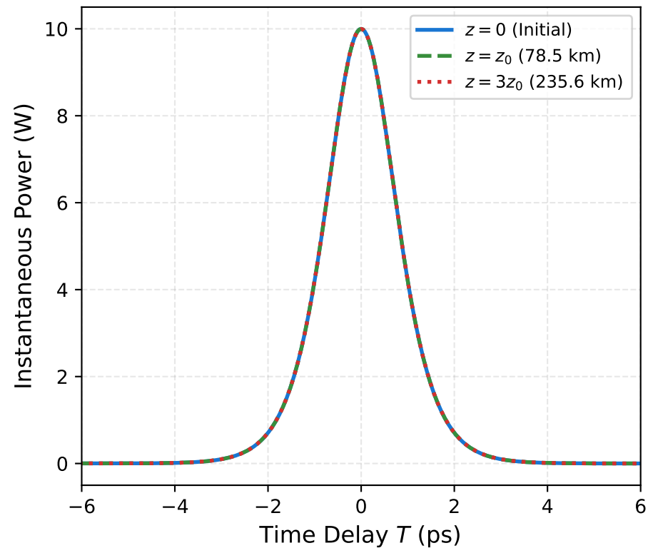
(a) Fundamental Soliton ( N = 1 )
