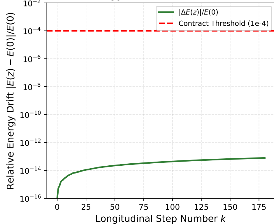
(c) Energy Conservation Invariant
