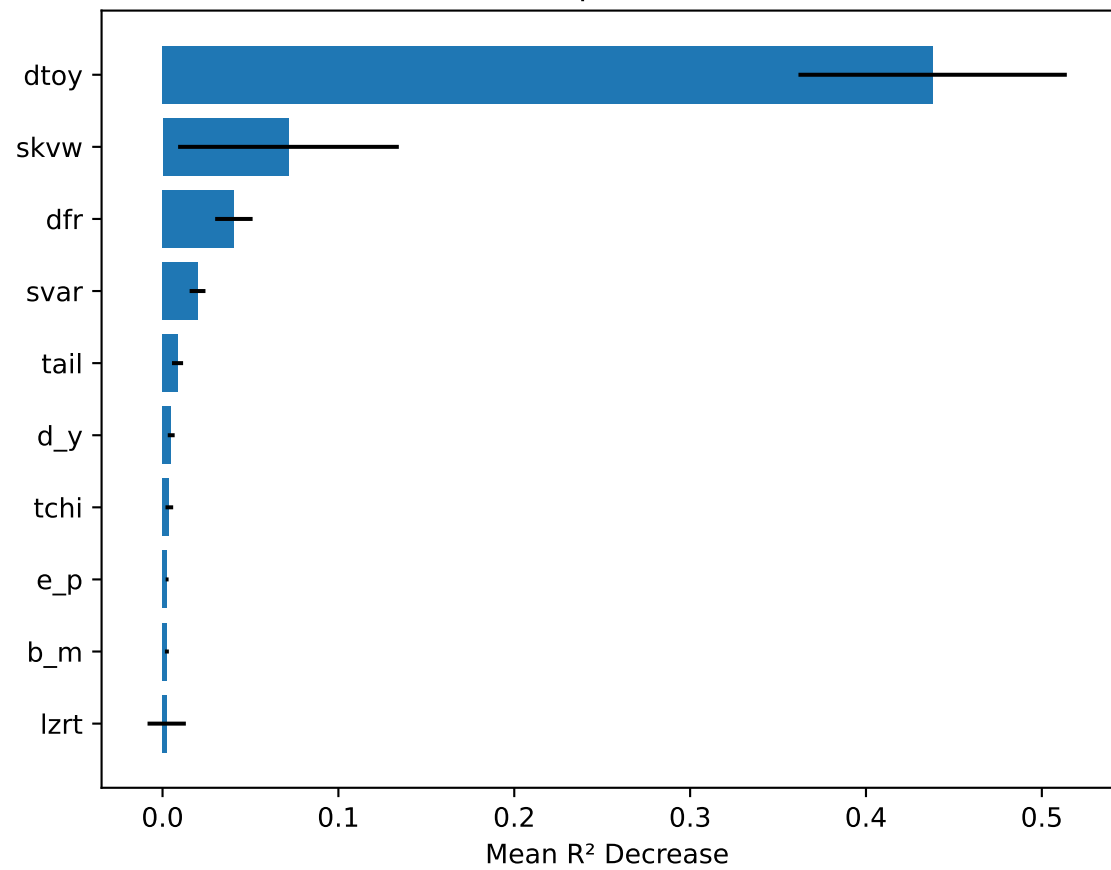
Permutation Importance (Test Set)
