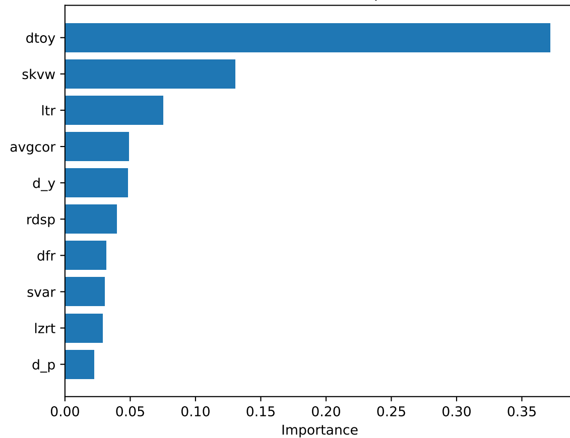
Tree-Based Feature Importance
