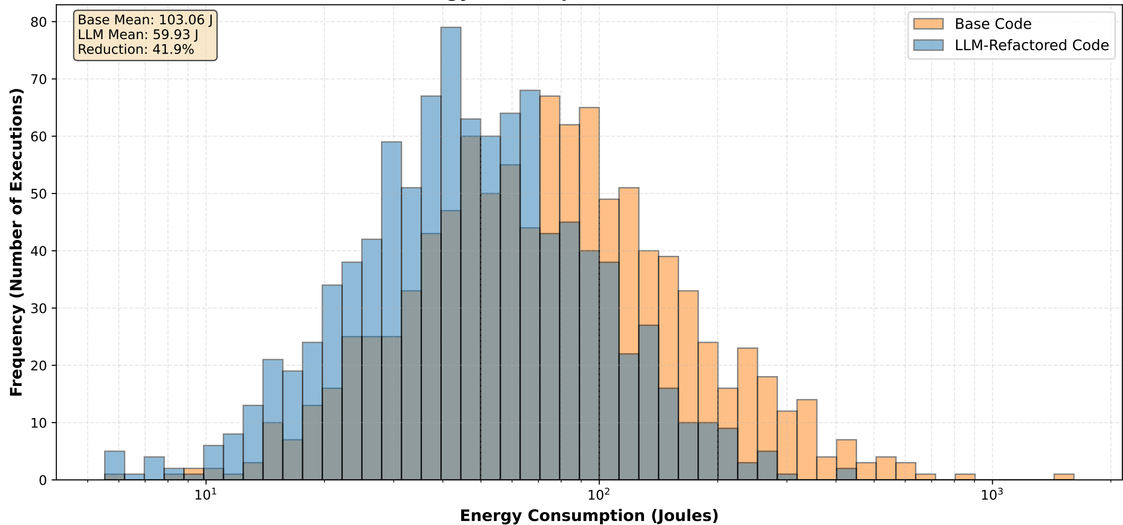
Distribution of Energy Consumption: Base vs LLM-Refactored Code
