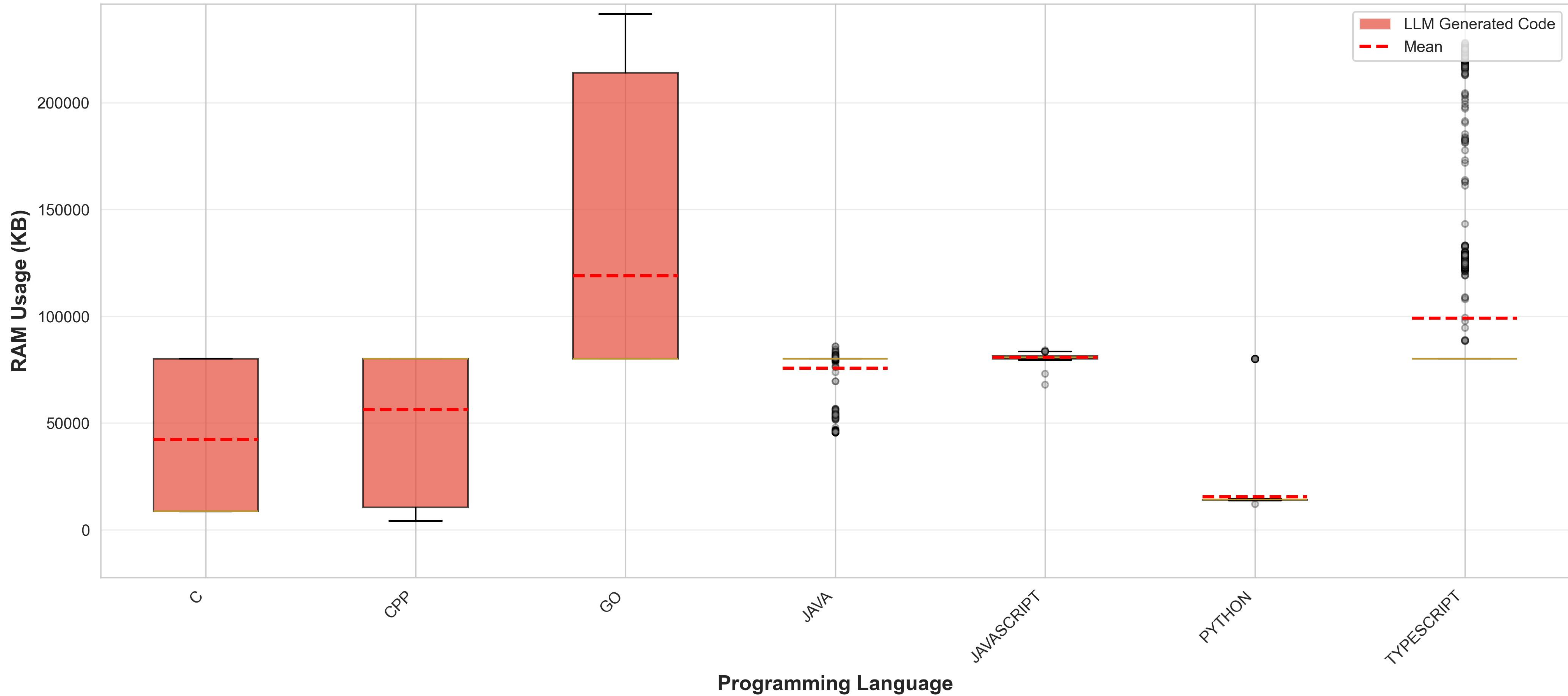
RAM Usage (KB) by Language - LLM Code (All LLM generated code)
