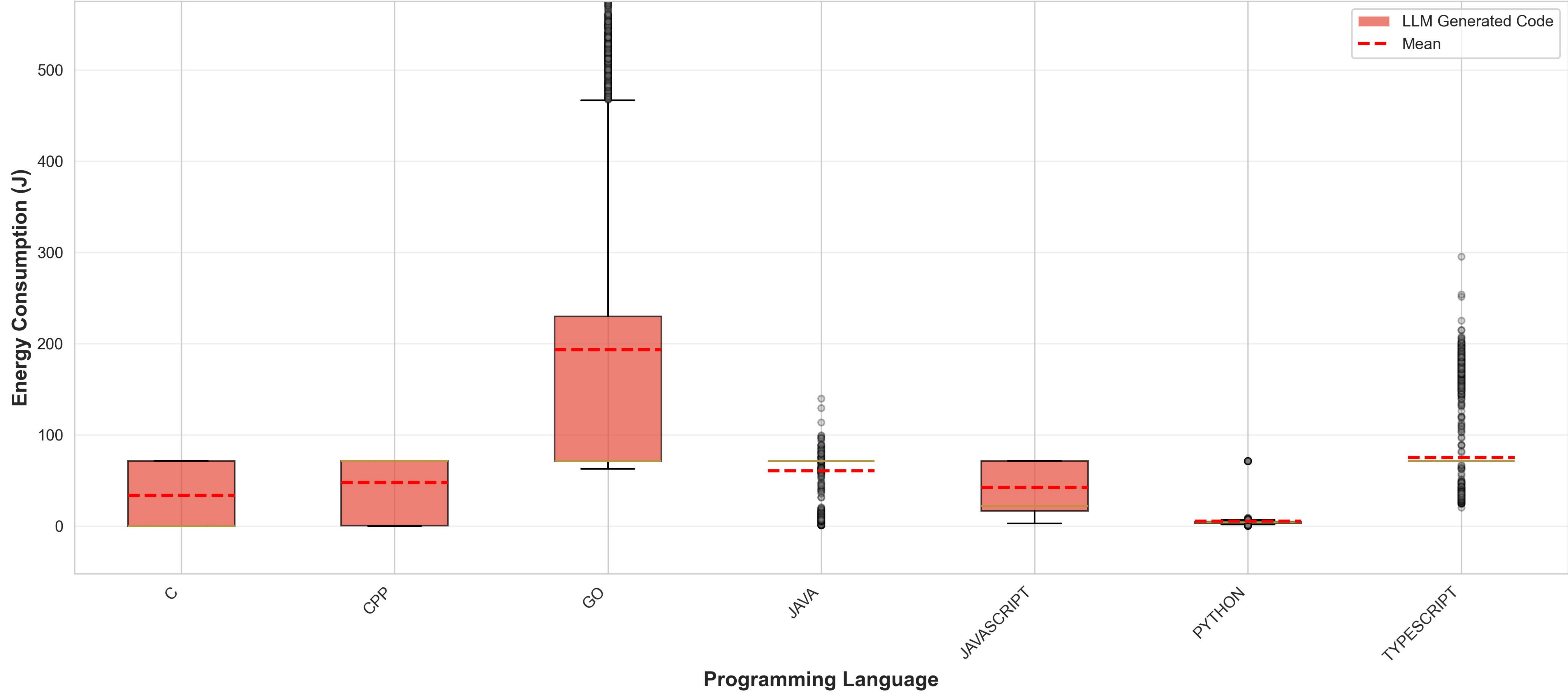
Energy Consumption (J) by Language - LLM Code (All LLM generated code)
