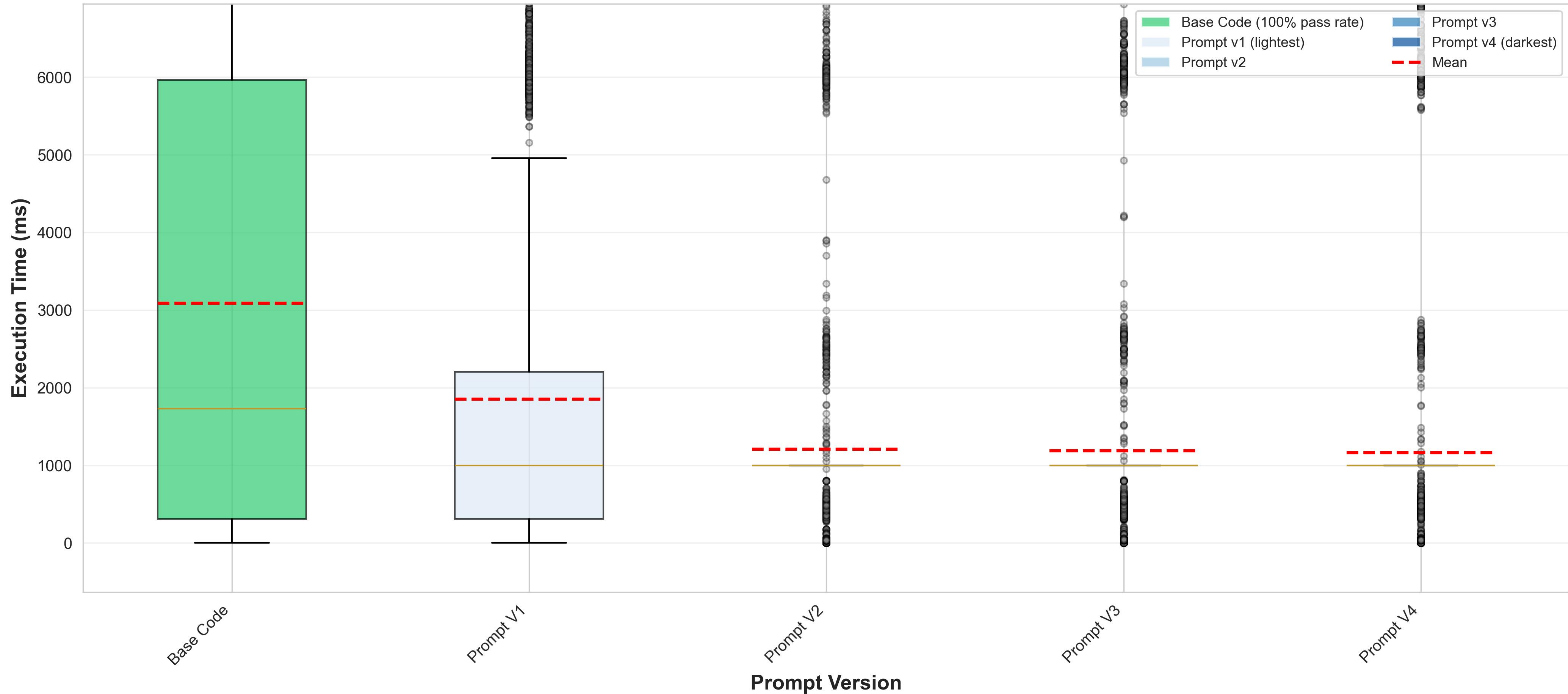
Execution Time (ms) by Prompt Version (Aggregated across all clusters - Base code with 100% pass rate only)
