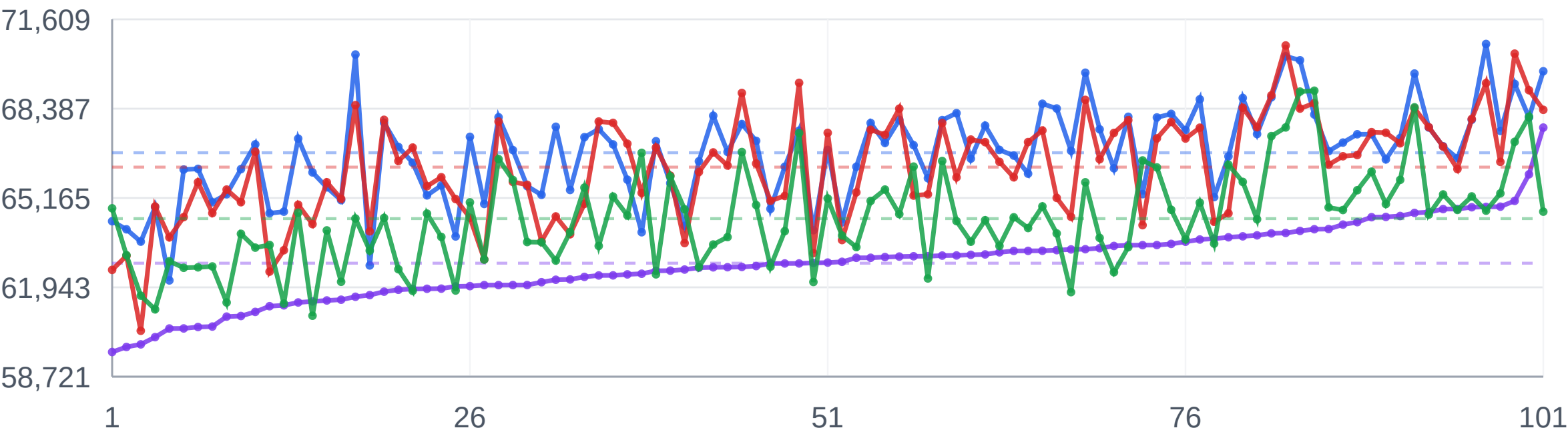
Final tour length by sorted run
