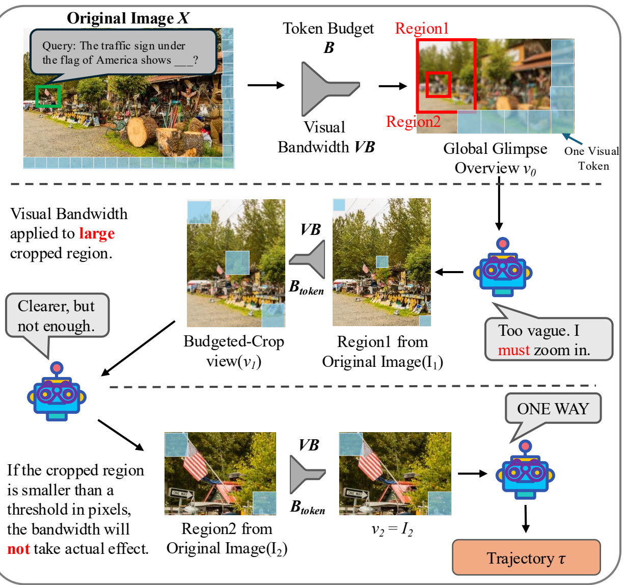
(a) Inference Pipeline Under Visual Bandwidth
