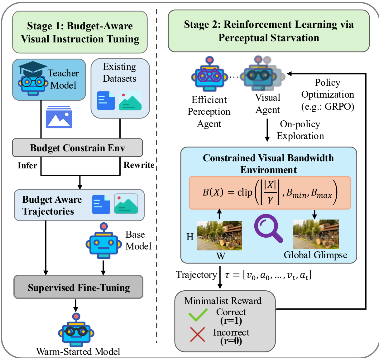
(b) Two Stage Training Pipeline
