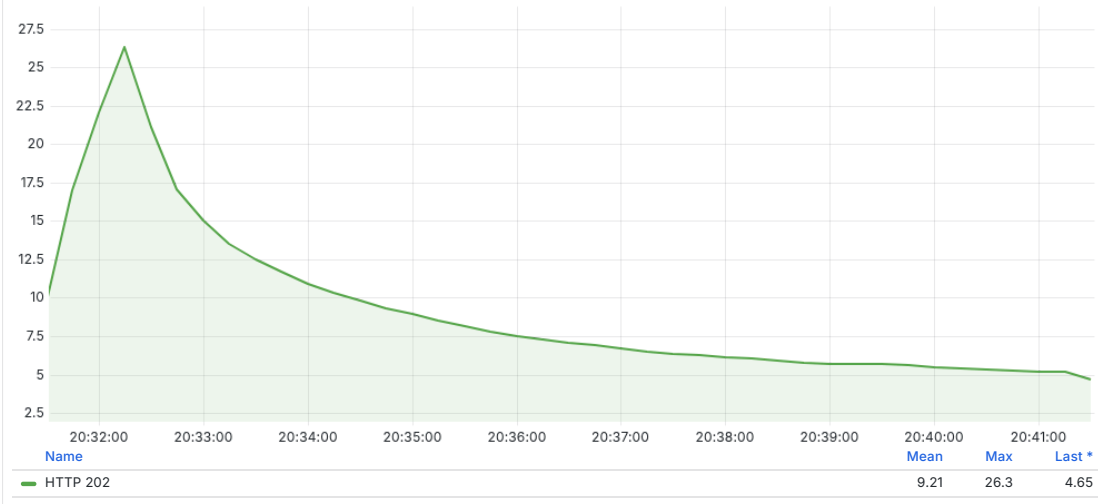
POST /inventory/reserve — Response Counts by Status
