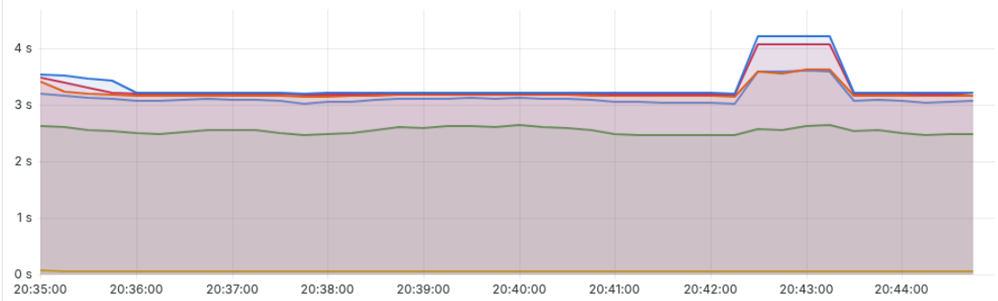
Order E2E Latency by Outcome — p50 / p95 / p99
