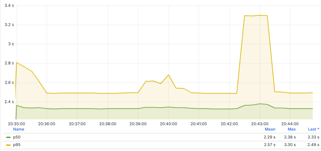
Order Queue Wait — p50 / p95
