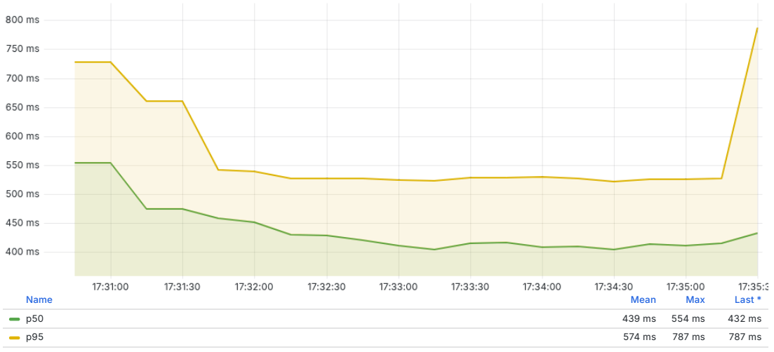
Order Processing Time — p50 / p95
