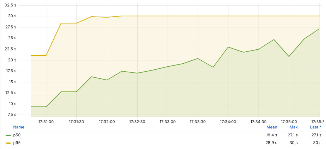
Order Queue Wait — p50 / p95
