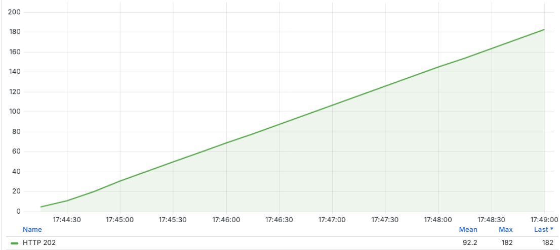
POST /inventory/orders — Response Counts by Status
