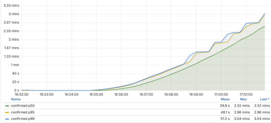
Order E2E Latency by Outcome — p50 / p95 / p99
