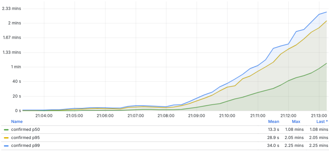
Order E2E Latency by Outcome — p50 / p95 / p99
