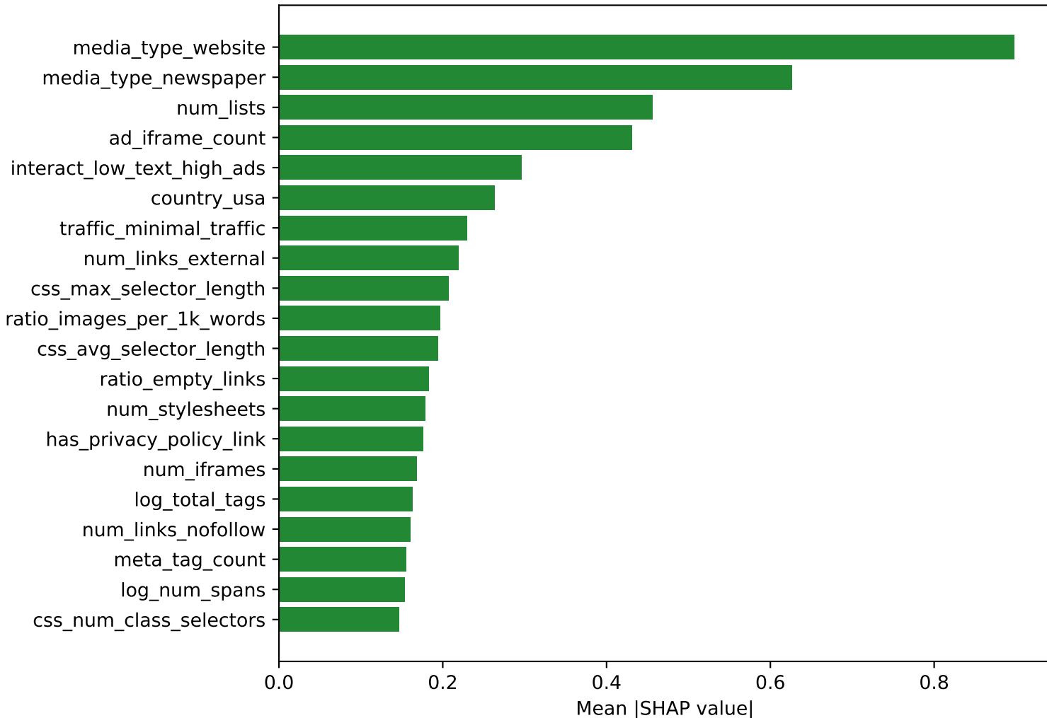
Top 20 Features - High Credibility (XGBoost SMOTE+weights, Enriched)
