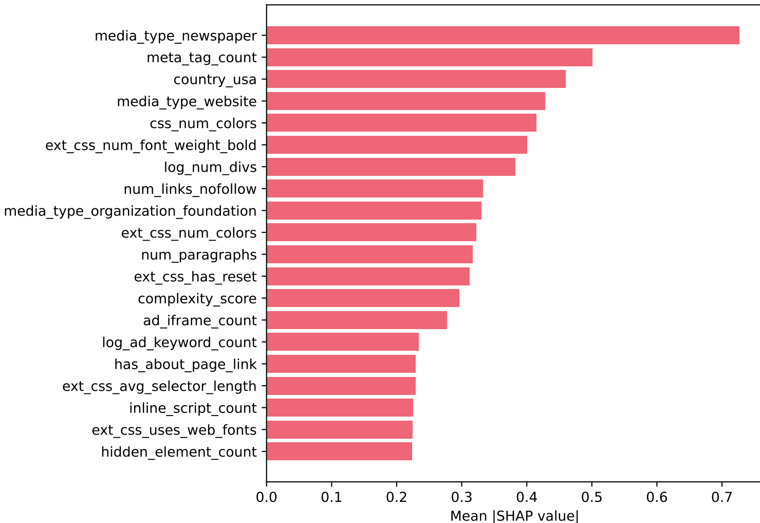
Top 20 Features - Low Credibility (XGBoost SMOTE+weights, Enriched)
