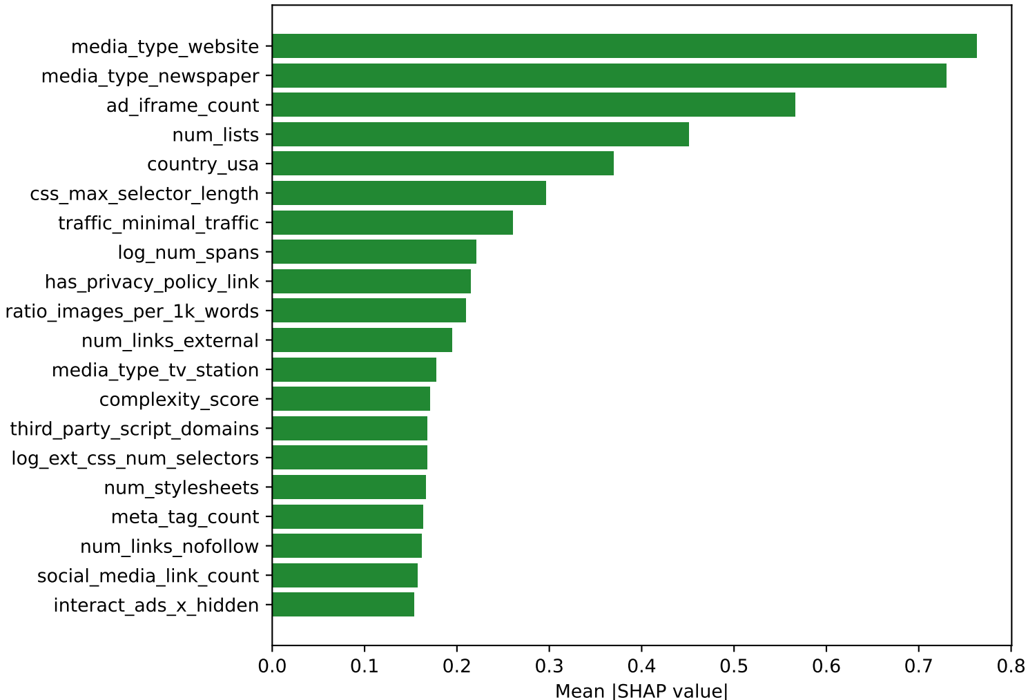
Top 20 Features - High Credibility (XGBoost SMOTE+weights, Enriched)
