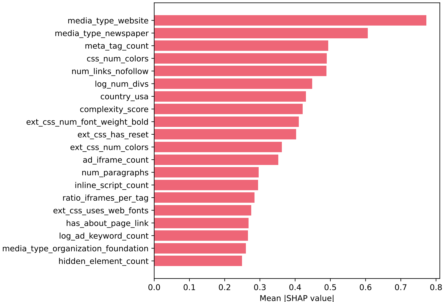
Top 20 Features - Low Credibility (XGBoost SMOTE+weights, Enriched)
