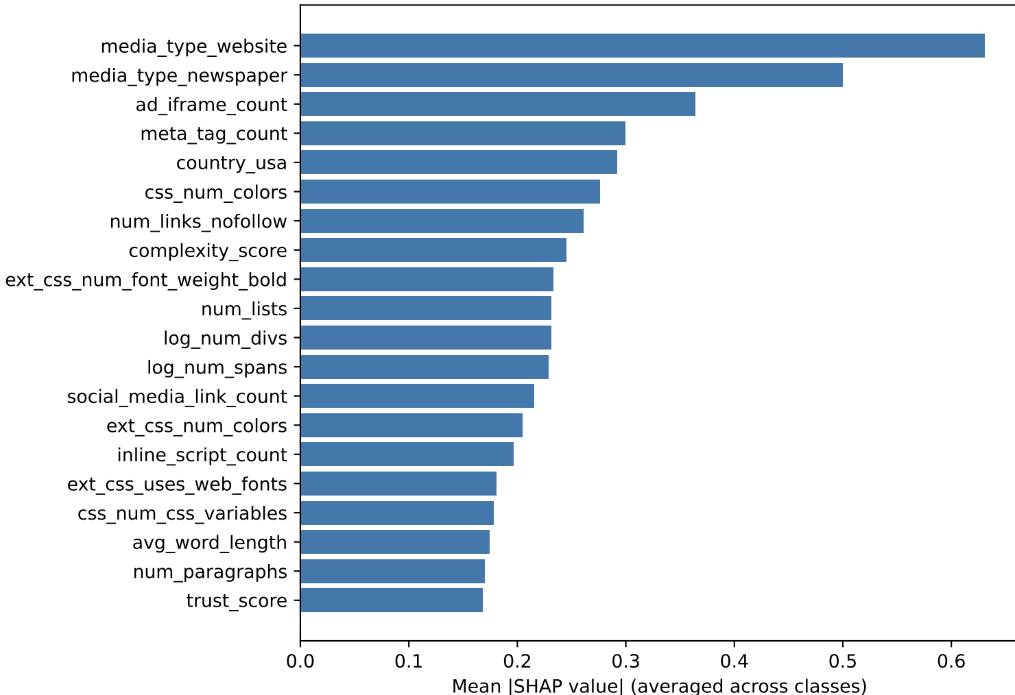
Top 20 Features - Overall Importance (XGBoost SMOTE+weights, Enriched)
