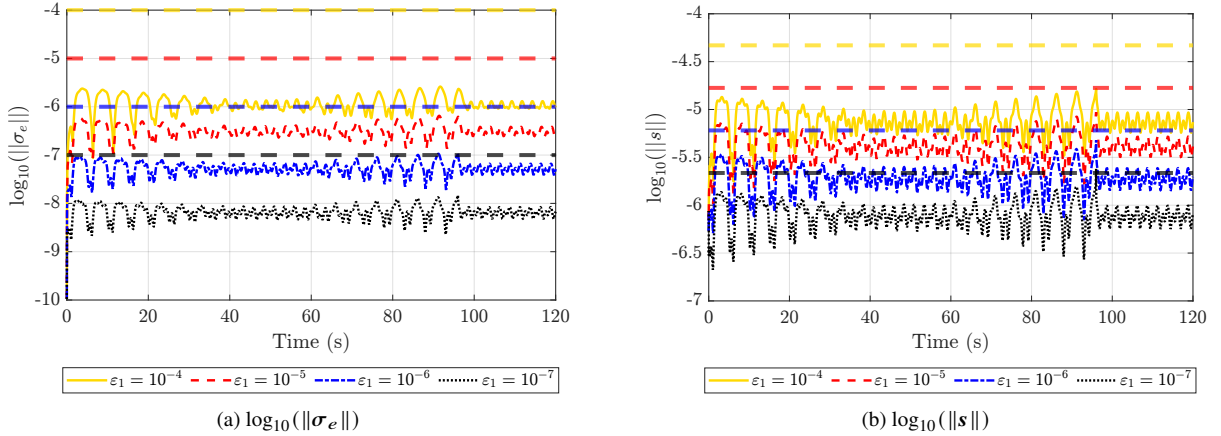
Fig. 6 Case 2: Log-scale error and sliding-variable norms for varying \varepsilon_1 .
