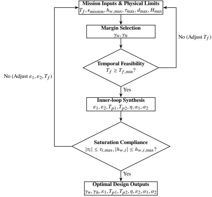
Fig. 1 Parameter-synthesis procedure.
