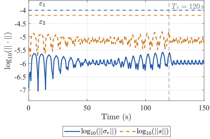
Fig. 3 Case 1: Log-scale tracking-error convergence.
