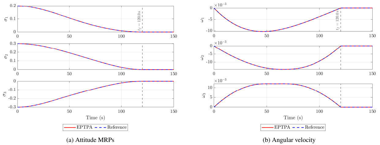
Fig. 3 Case 1: Reference tracking in MRPs and angular rates.
