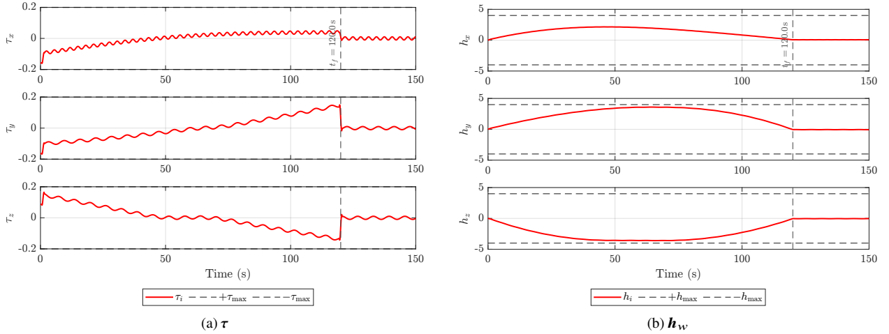
Fig. 7 Case 1: Torque and wheel momentum under the beyond-bound transient disturbance.
