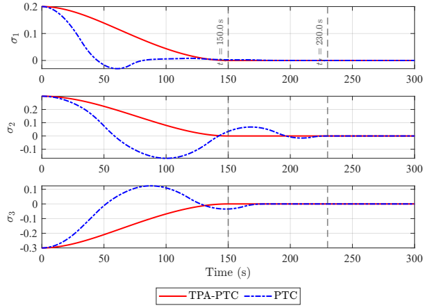
(c) Attitude error ( T_f = 150 s)
