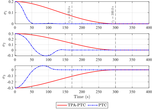
(a) Attitude error ( T_f = 300 s)
