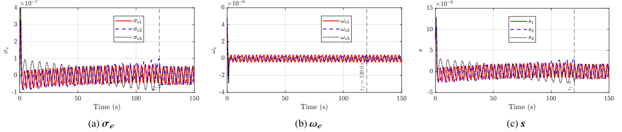
Fig. 6 Case 1: Error convergence under beyond-bound transient disturbance.
