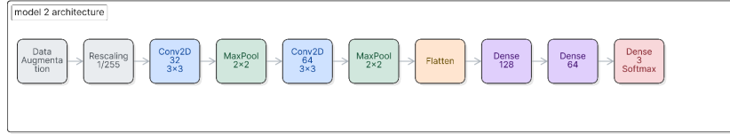
Fig. 3. Architecture of the second CNN model.
