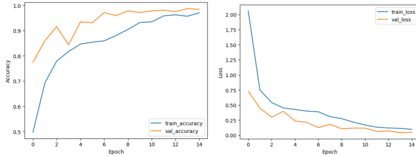
Fig. 7. Training and validation accuracy and loss curves for Model 3.
