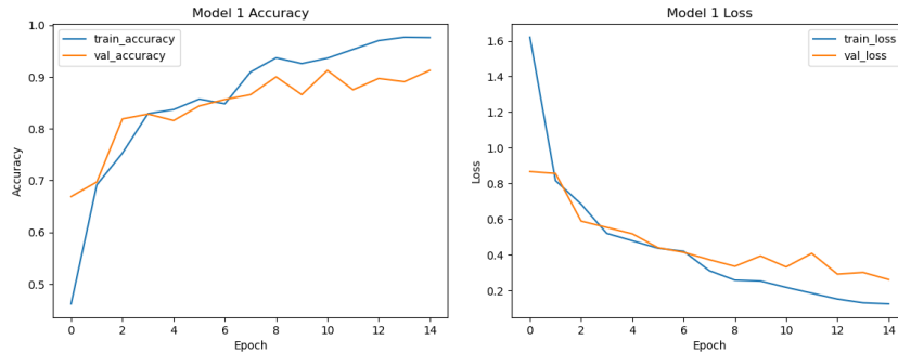
Fig. 5. Training and validation accuracy and loss curves for Model 1.
