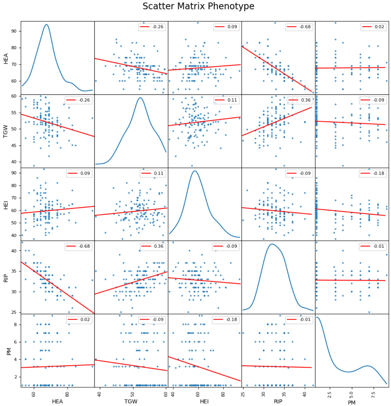
Fig. 1: Scatter matrix of phenotype data.
