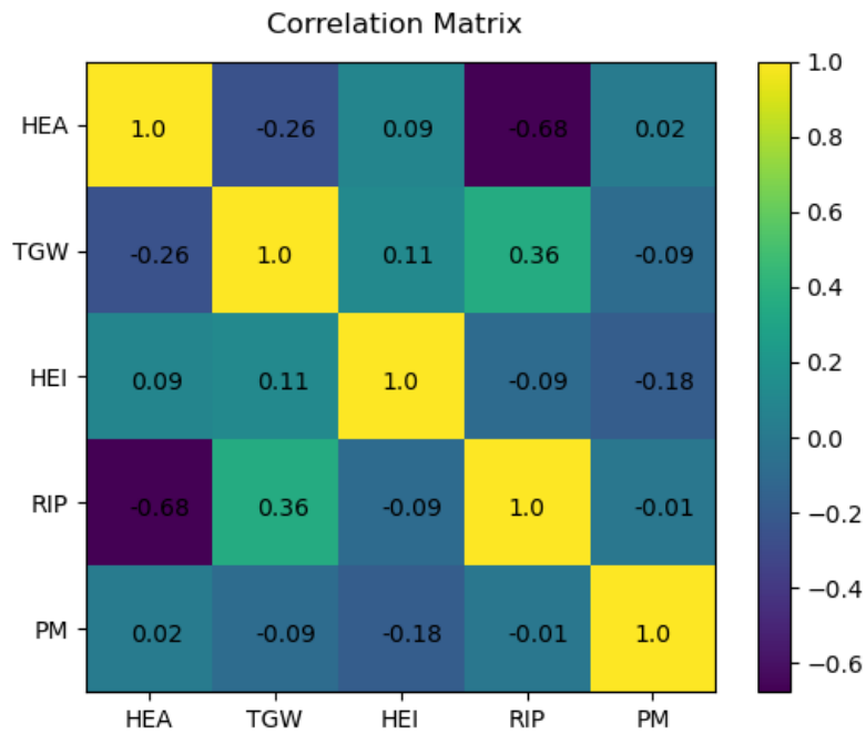
Fig. 2: Correlation matrix of phenotype data.
