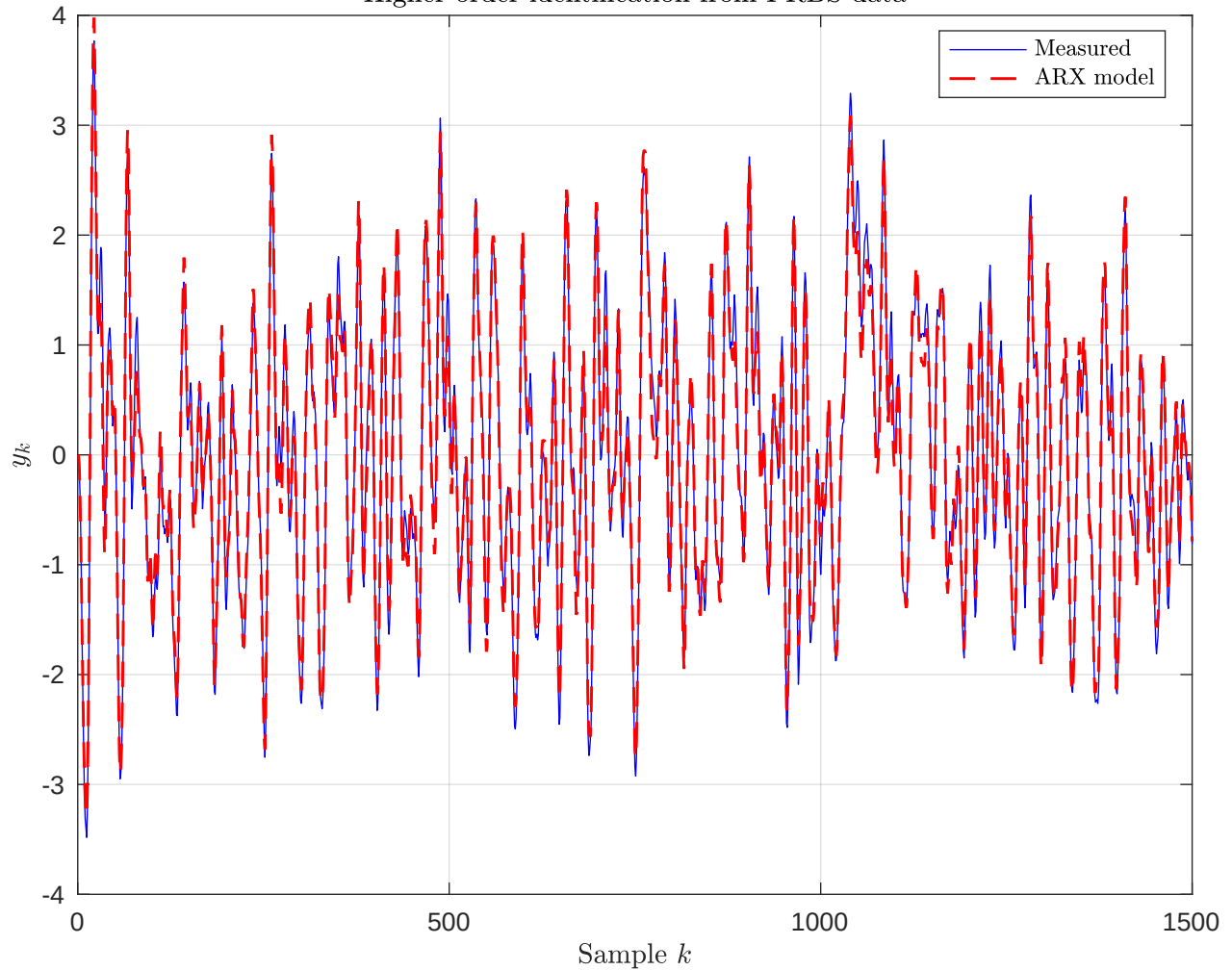
Higher-order identification from PRBS data
