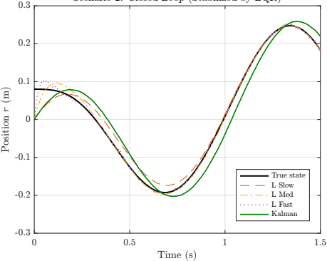
Scenario 2: Closed-Loop (Stabilized by LQR)
