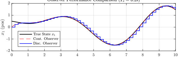
Observer Performance Comparison ( T_s = 0.2\text{s} )
