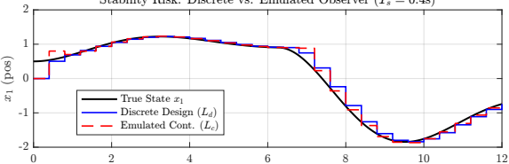
Stability Risk: Discrete vs. Emulated Observer ( T_s = 0.4\text{s} )
