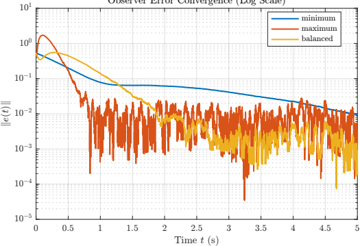
Observer Error Convergence (Log Scale)
