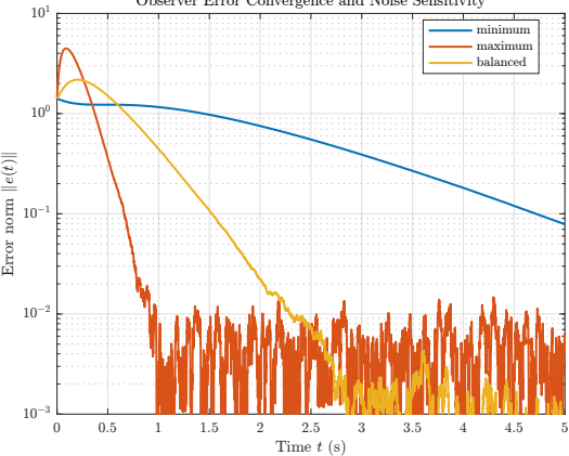
Observer Error Convergence and Noise Sensitivity
