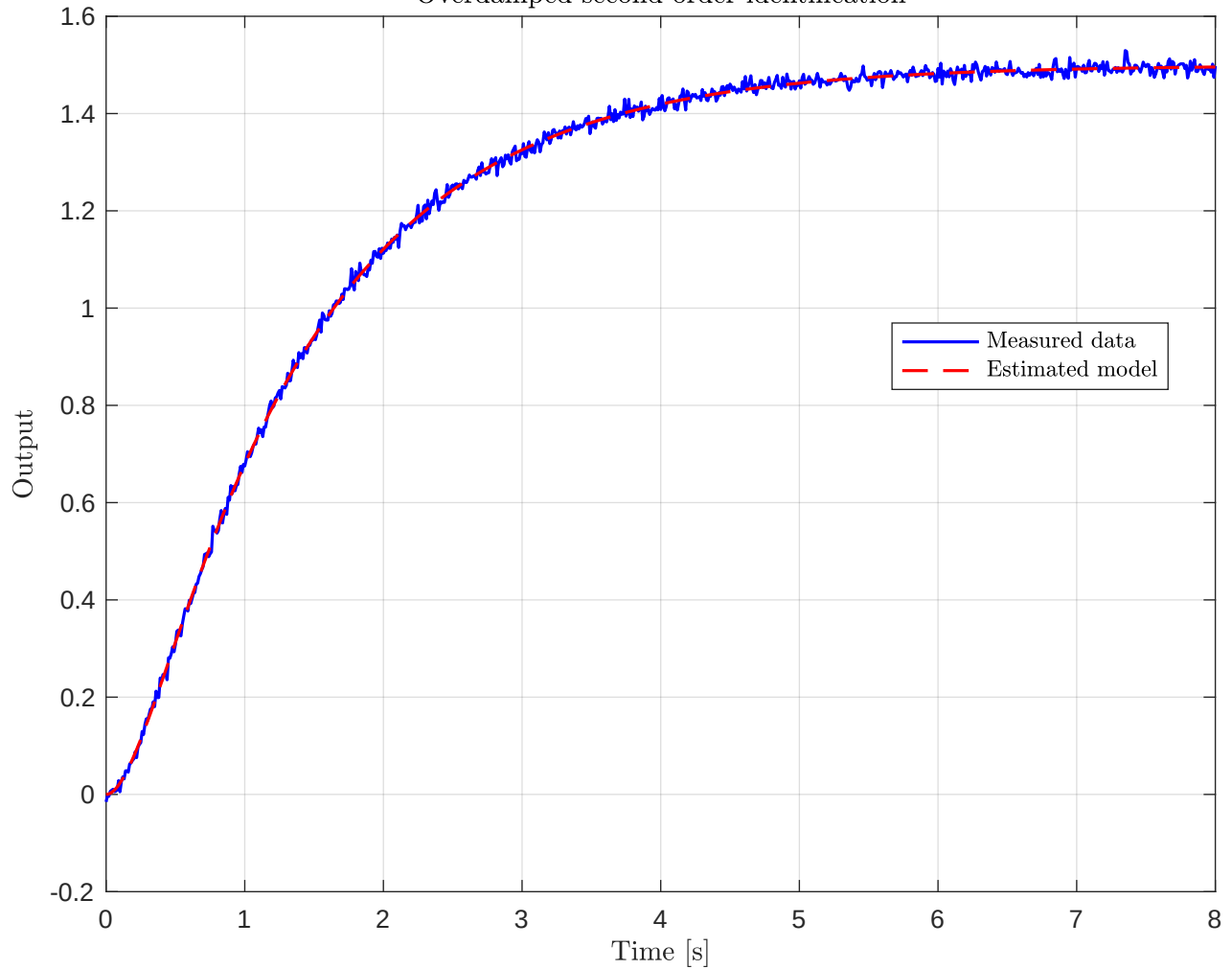
Overdamped second-order identification
